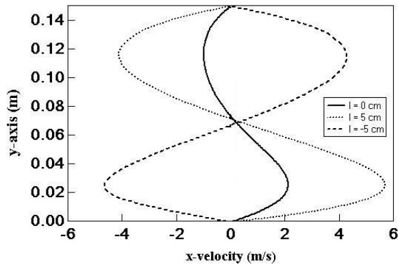
Fig.14 Velocity profile in x-velocity when consider y-axis at center of swirling flow.
