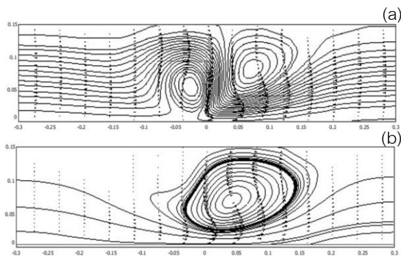
Fig.9 Swirling flow of WP at u = 0.5 m/s; h = 2 cm and (b) h = 6 cm.
