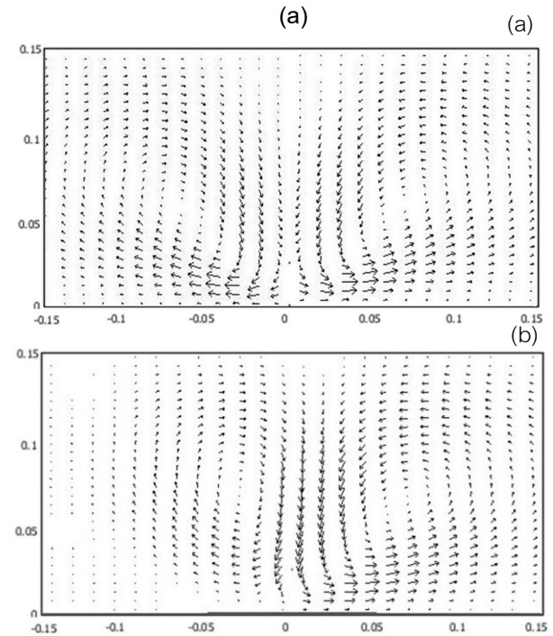
Fig.7 Velocity vector under electric field when u = 0 m/s at h = 2 cm; (a) WW (b) WP.
