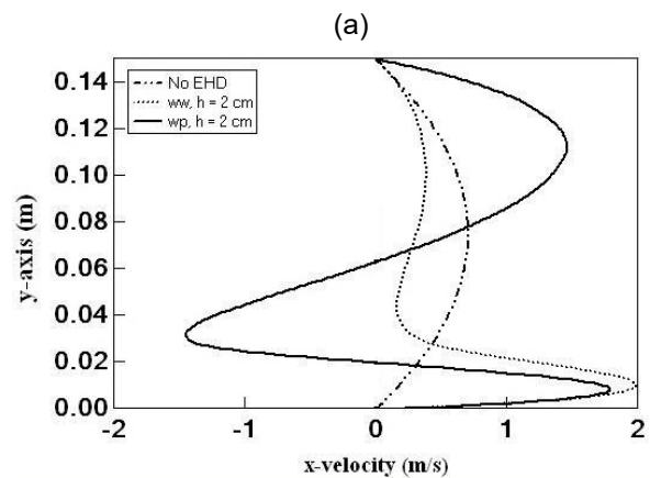
Fig.10 x-velocity profile when consider y -axis at x = 0 m.
