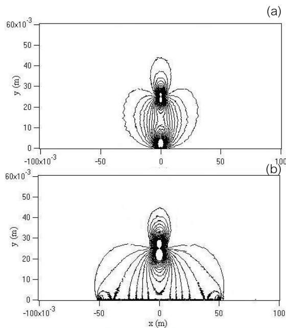
Fig.6 Electric force at h = 2 cm; WW (b) WP.
