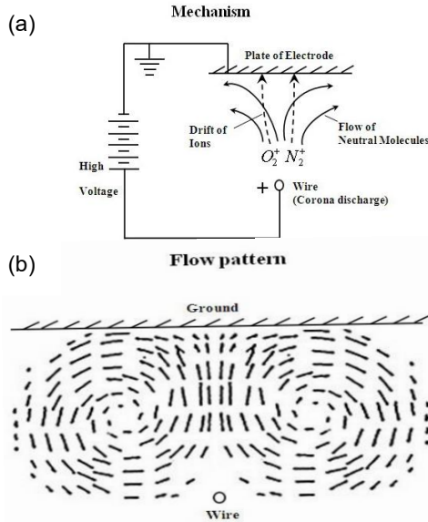
Fig.1 Electrohydrodynamic method [8].
