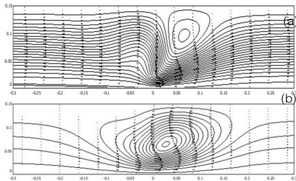
Fig.8 Swirling flow of WW at u = 0.5 m/s; (a) h = 2 cm and (b) h = 6 cm.
